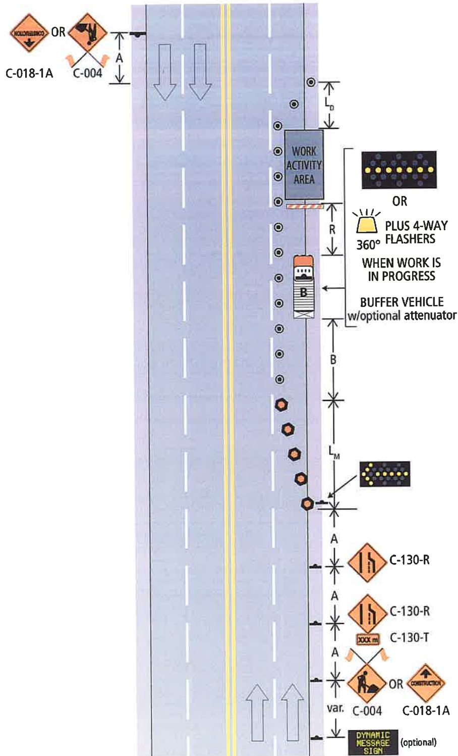
Figure 8.6: Right Lane Closed – Short and Long Duration
